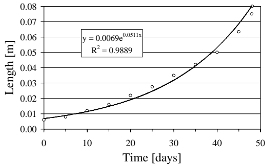
Figure 2: Velocity of growth of the preferential flow path. Breakthrough occurs after 48 days.
