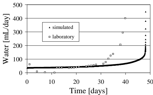
Figure 3: Rate of water in mL per day flooded through the core during the numerical and laboratory experiment.
