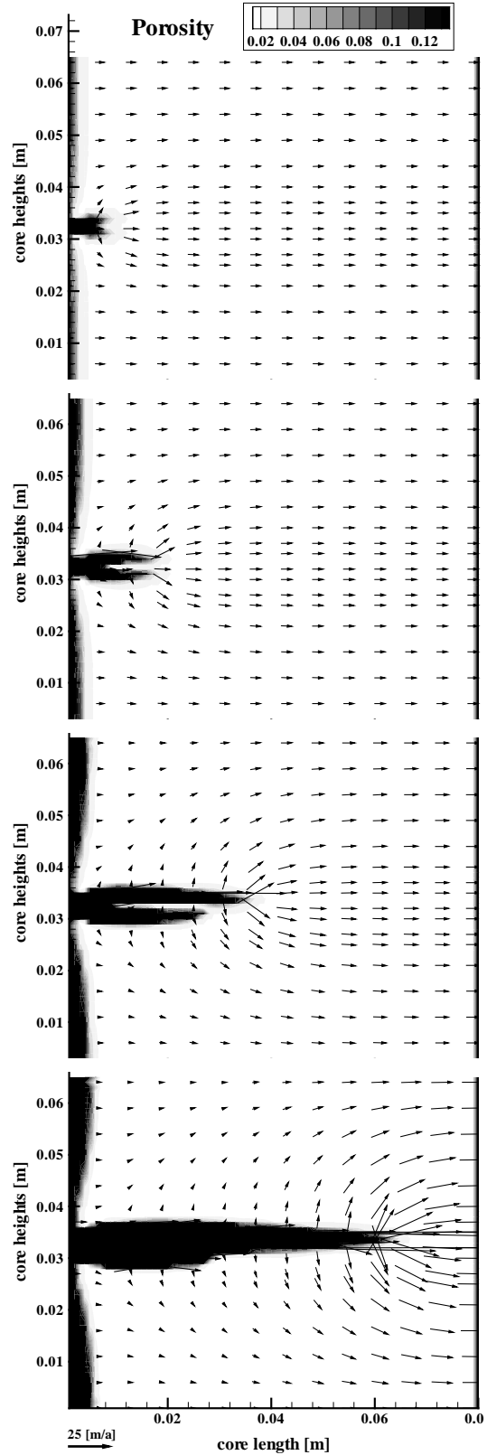
Figure 1: Development of porosity during the numerical core flooding experiment. From top to bottom, distribution after 5, 15, 30, and 45 days. Arrows depict direction and magnitude of flow
