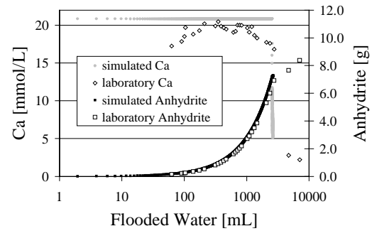
Figure 5: Comparison of laboratory and simulated data of the concentration of calcium in the solution and the total amount of anhydrite dissolved during the simulation dependent on the amount of water flooded through the core.
